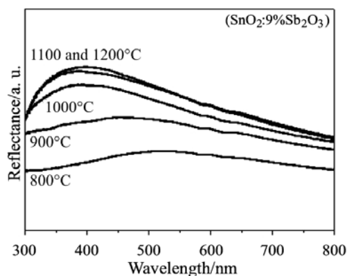
Fig. 3 Diffuse reflectivity data of the SnO 2 ·9%Sb 2 O 3 system, as a function of the heat-treatment temperature in an air environment
